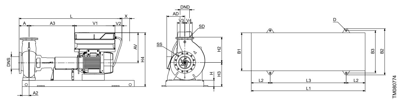
EN/ISO base frame with 4 mounting holes, center outlet
