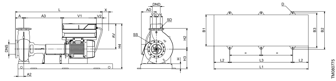
EN/ISO base frame with 6 mounting holes, center outlet
