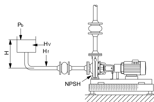
Suction lift with negative H
