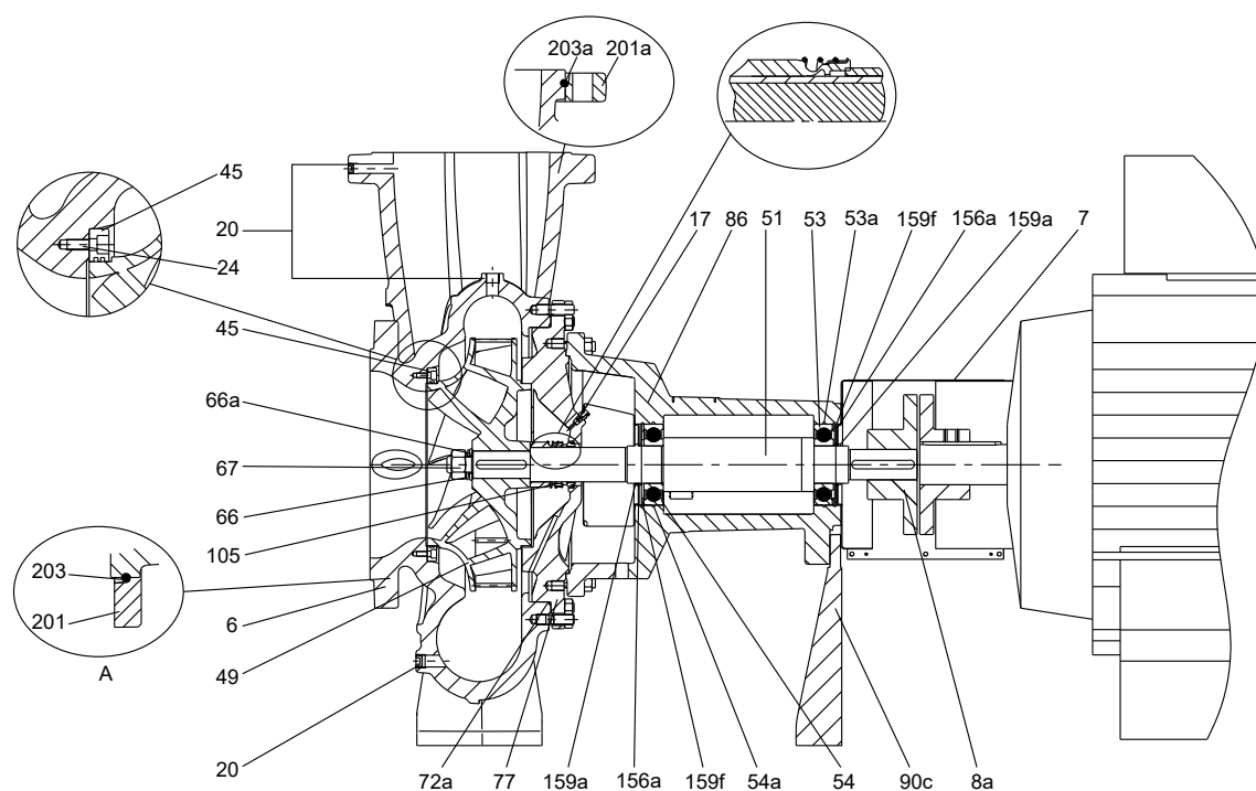
Sectional drawing, tangential outlet, DN 200 and DN 250
