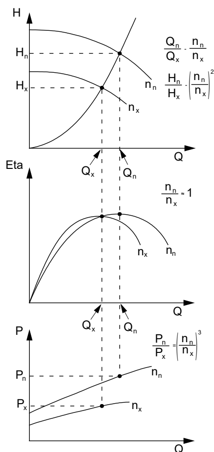
Affinity equations
