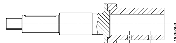
2-part stub shaft, NB pump
