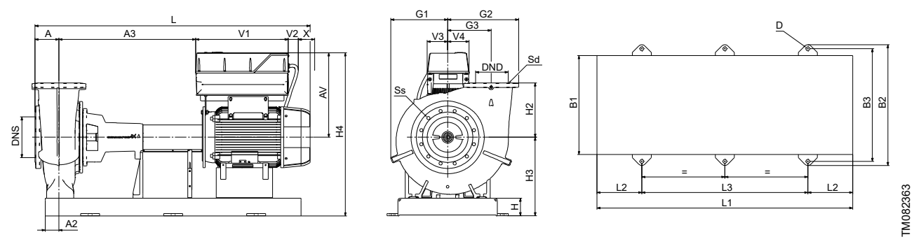
EN/ISO base frame with 6 mounting holes, tangential outlet
