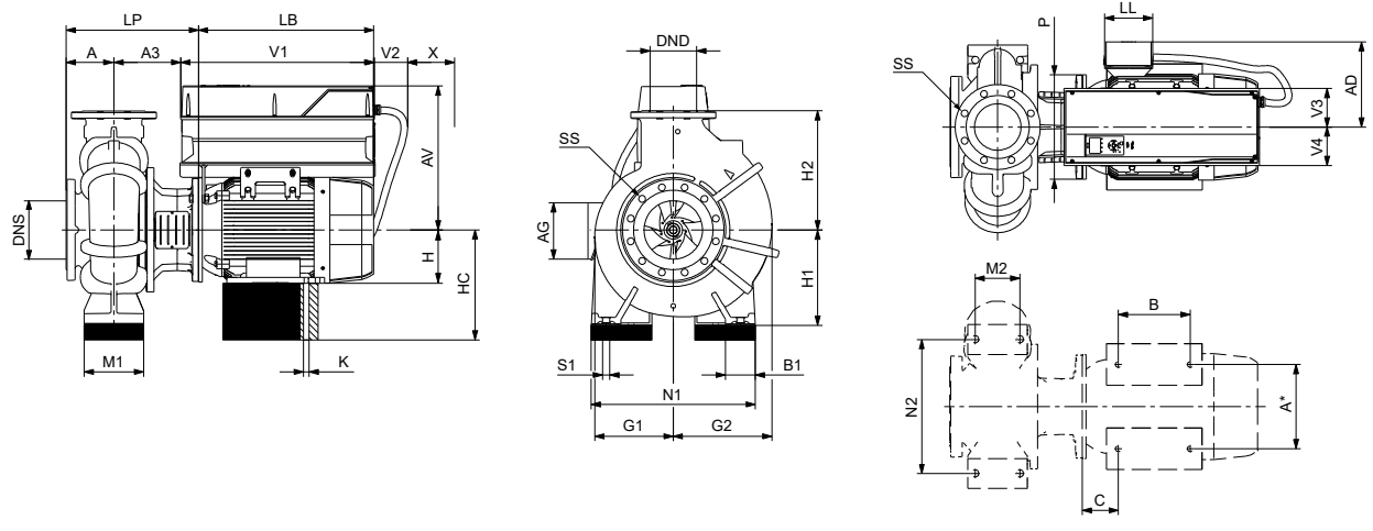
Mounting design C1 with support blocks under the motor and pump housing (Variant 3 in section Support blocks)
