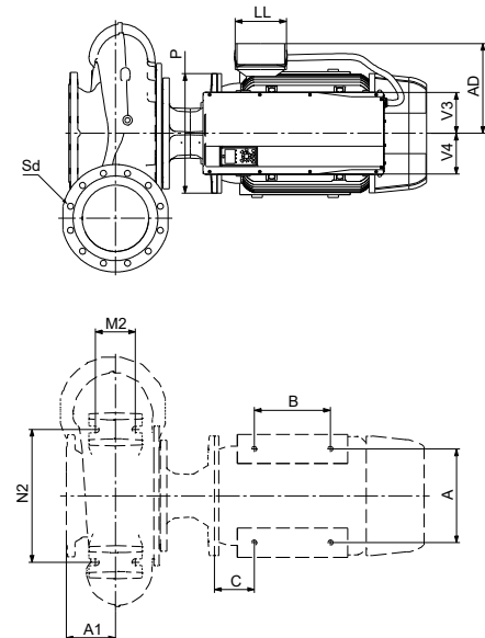
Mounting design C2, with support blocks under the motor (Variant 1b in section Support blocks)
