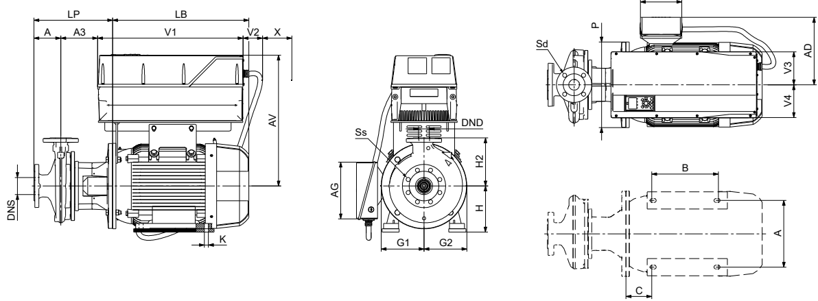
Mounting design B, with support blocks under the motor (Variant 1a in section Support blocks)
